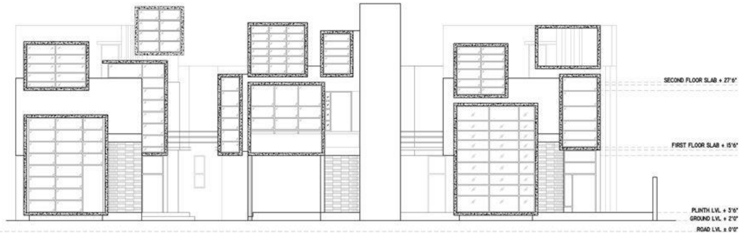
NORTH ELEVATION
