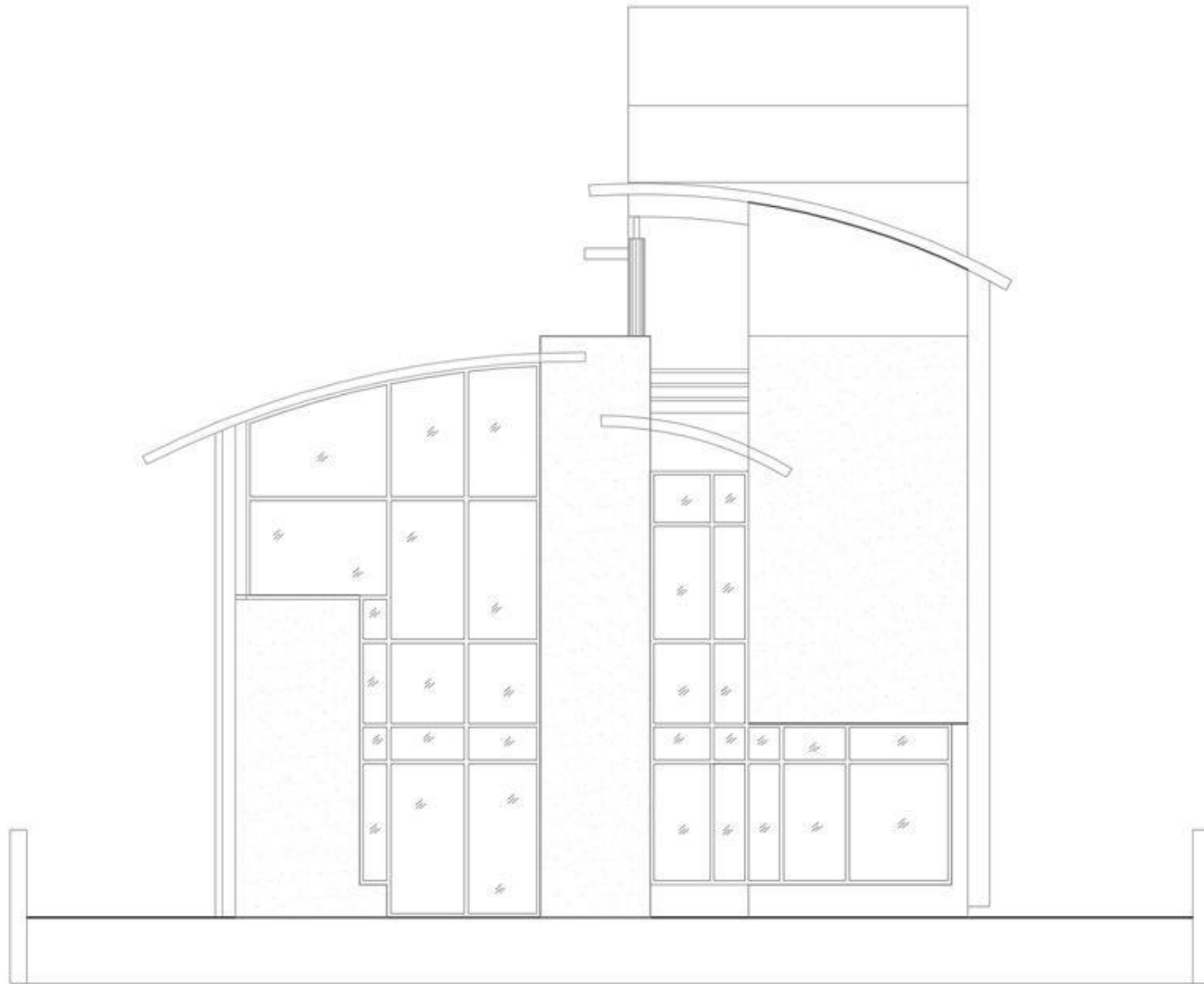
WEST FRONT ELEVATION
